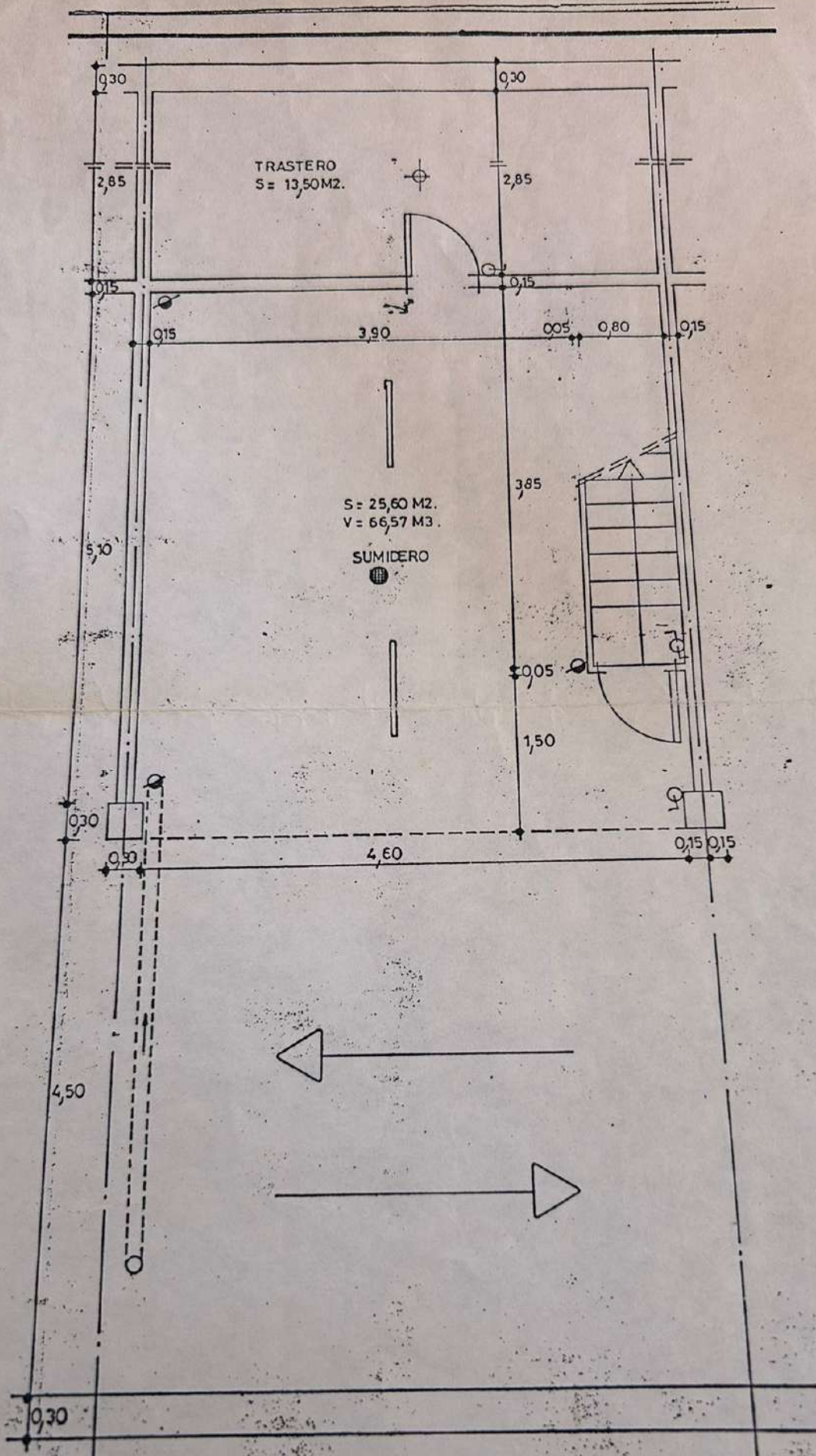
PLANTA SOTANO SUP. CONST. = 66,85 M 2 .
