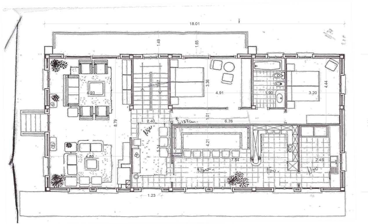
EXISTING GROUND FLOOR * MEASUREMENTS IN METERS
