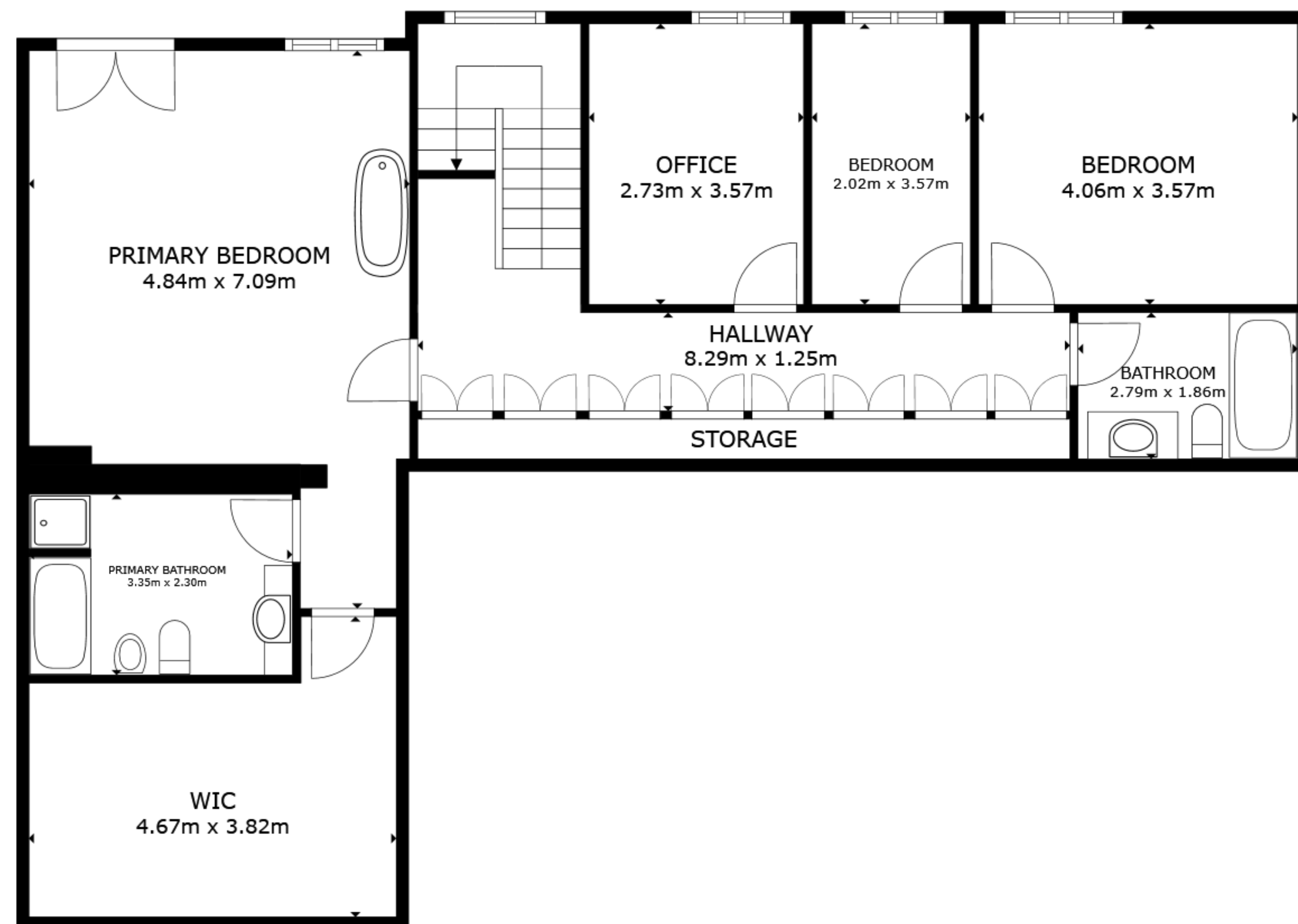
FLOOR 1
