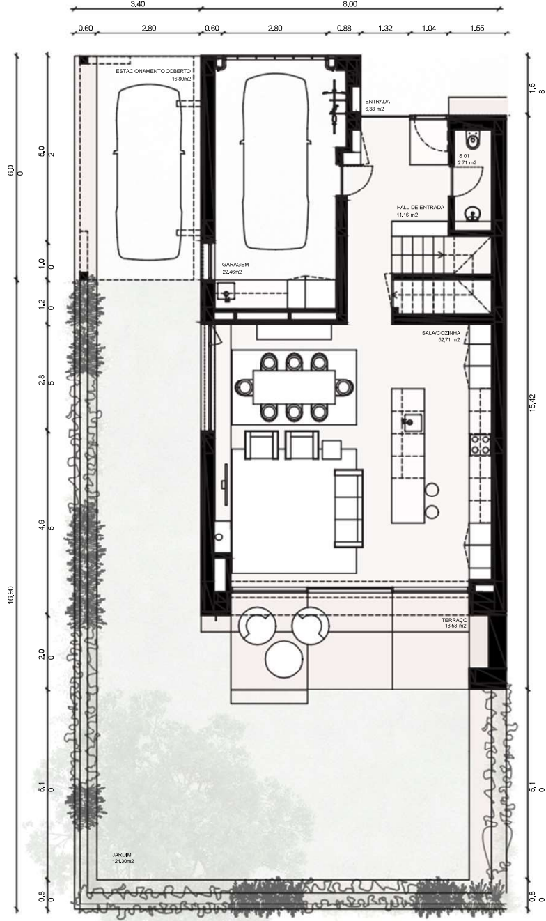
PISO TÉRREO | GROUND FLOOR
