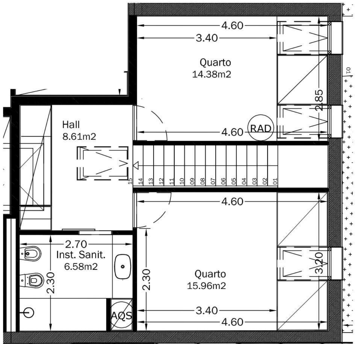
T2 O Duplex PISO 5 2 BED, O Duplex 5TH FLOOR
