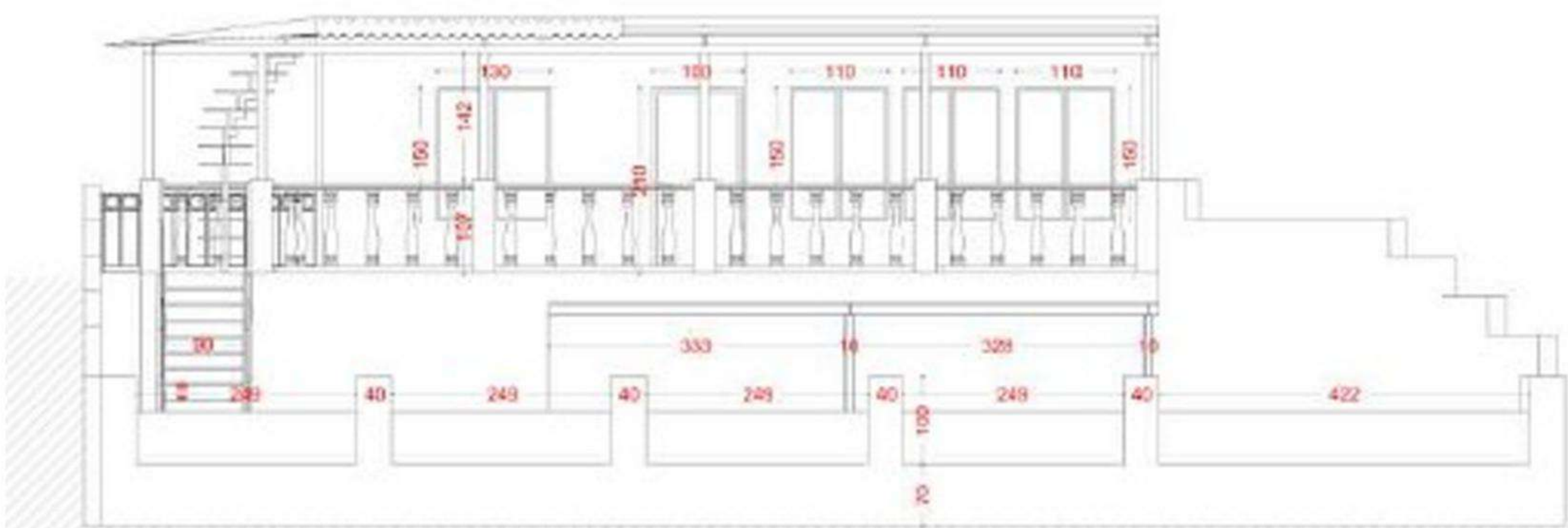
ALZADO NORTE NORTH ELEVATION
