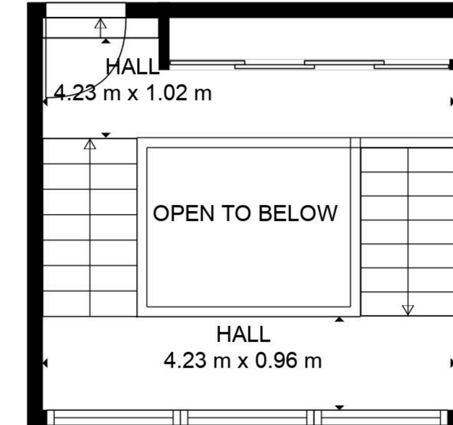
FLOOR 3
