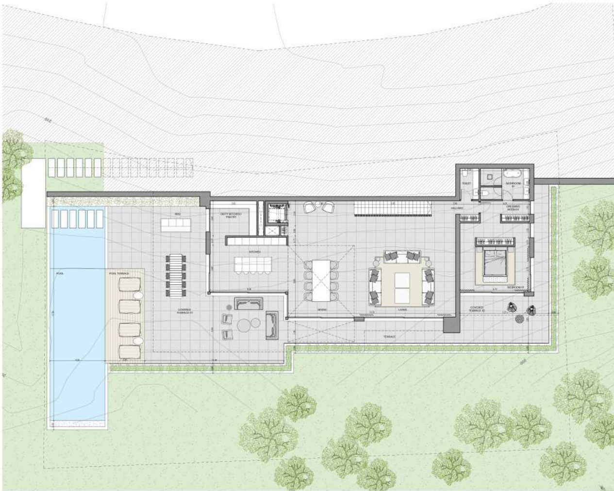
VILLA 04 GROUND FLOOR
