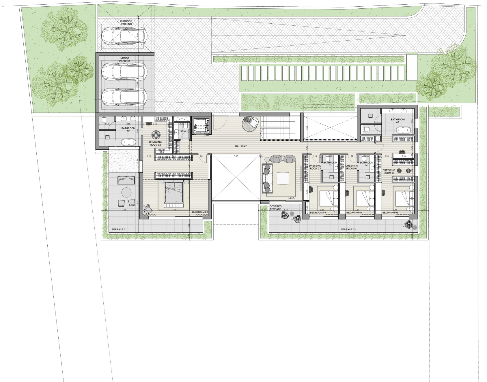
VILLA 02 FIRST FLOOR
