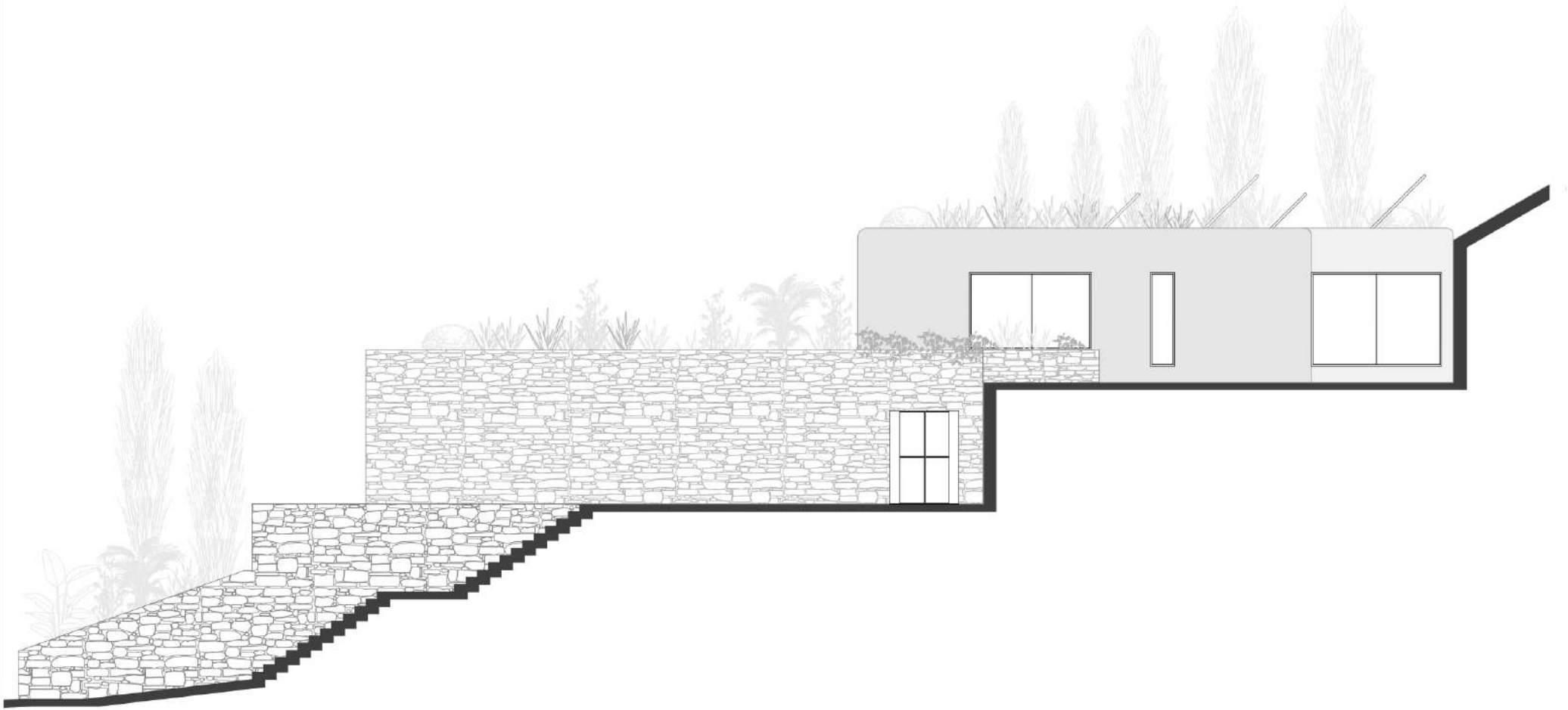
South elevation
