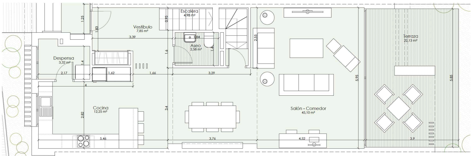
Ground Floor with garden
