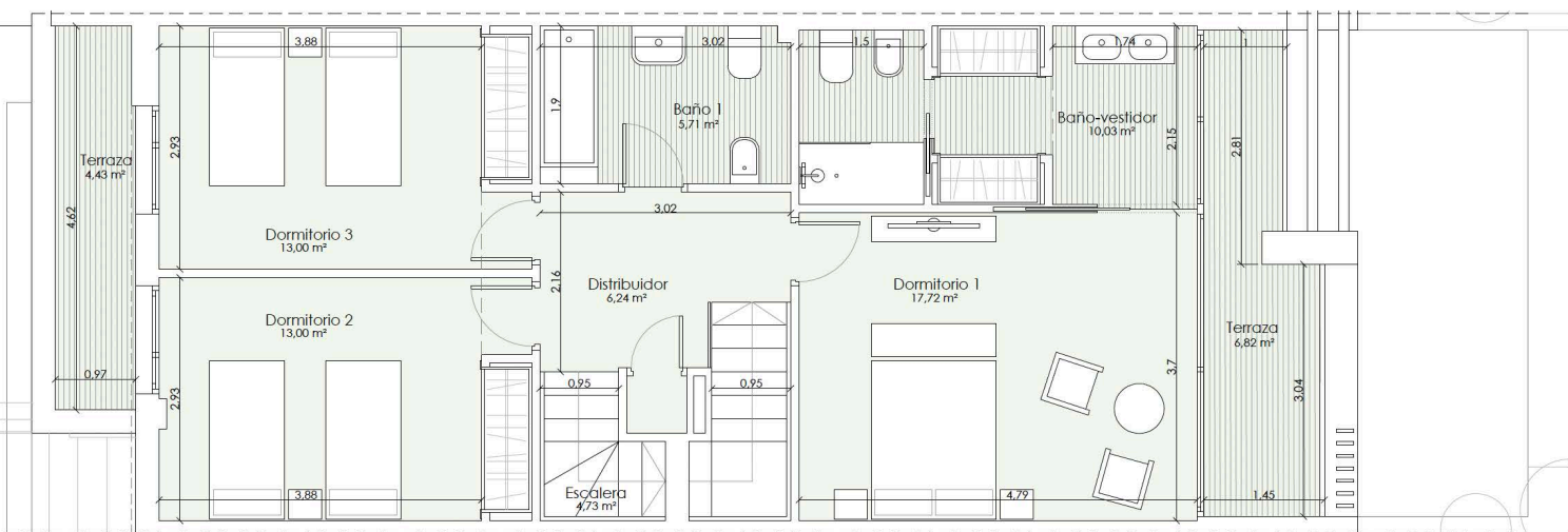
First Floor with balcony
