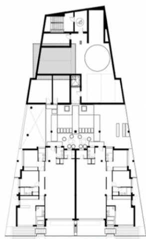
GARAGE floor -2
