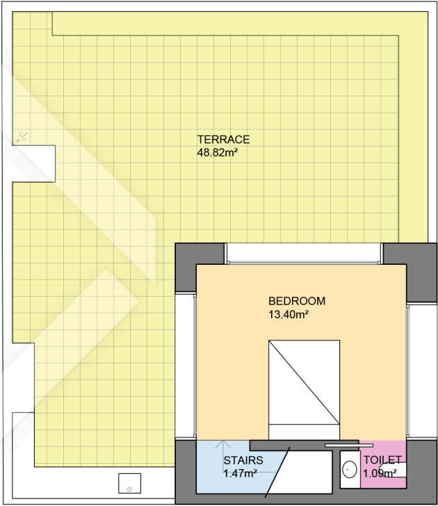
UPPER FLOOR Height = 2.57m
