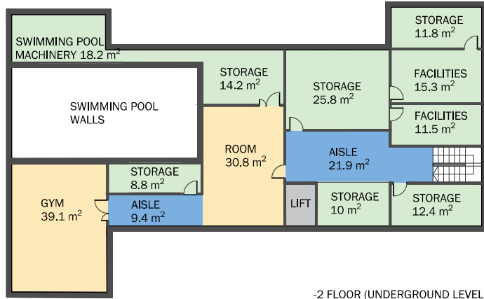
-2 FLOOR (UNDERGROUND LEVEL)
