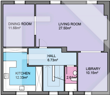
First floor h = 2.60m
