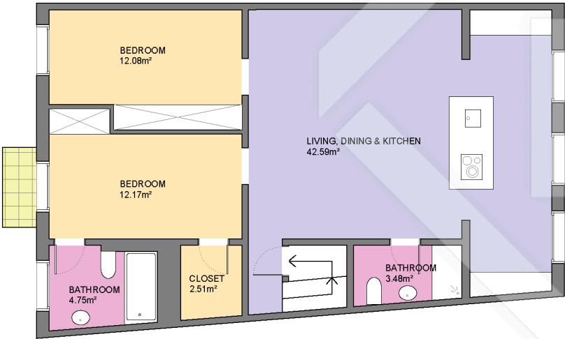
SECOND FLOOR
