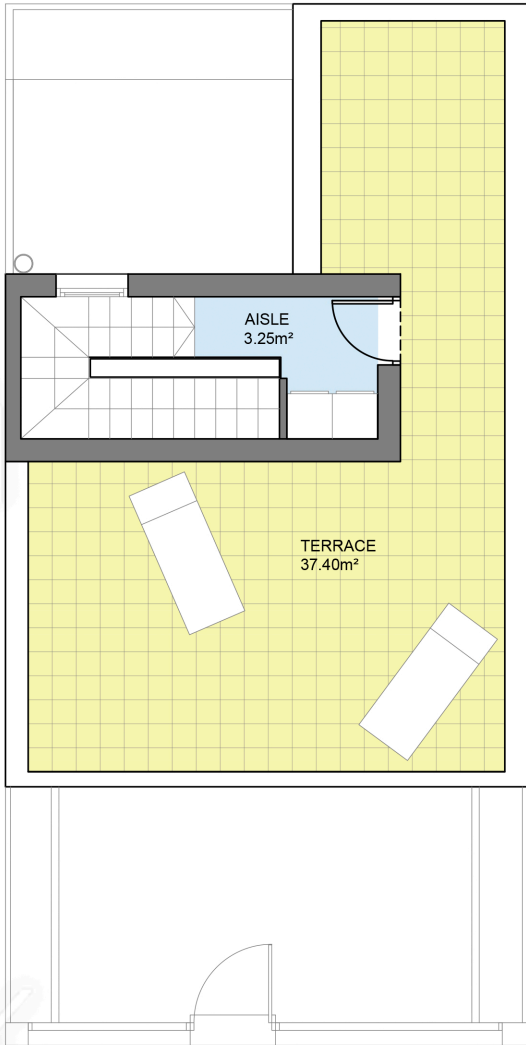
ATTIC FLOOR
