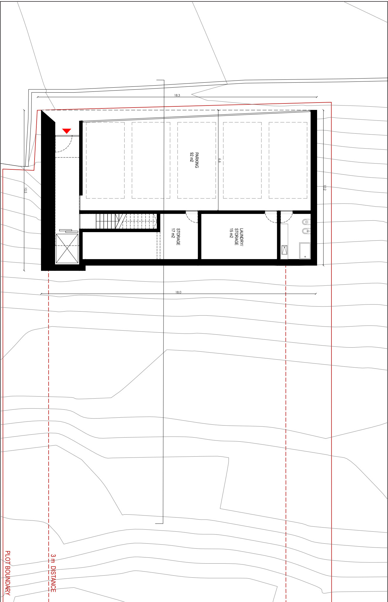
PLAN 0 - 1:100 surface 197 m 2
