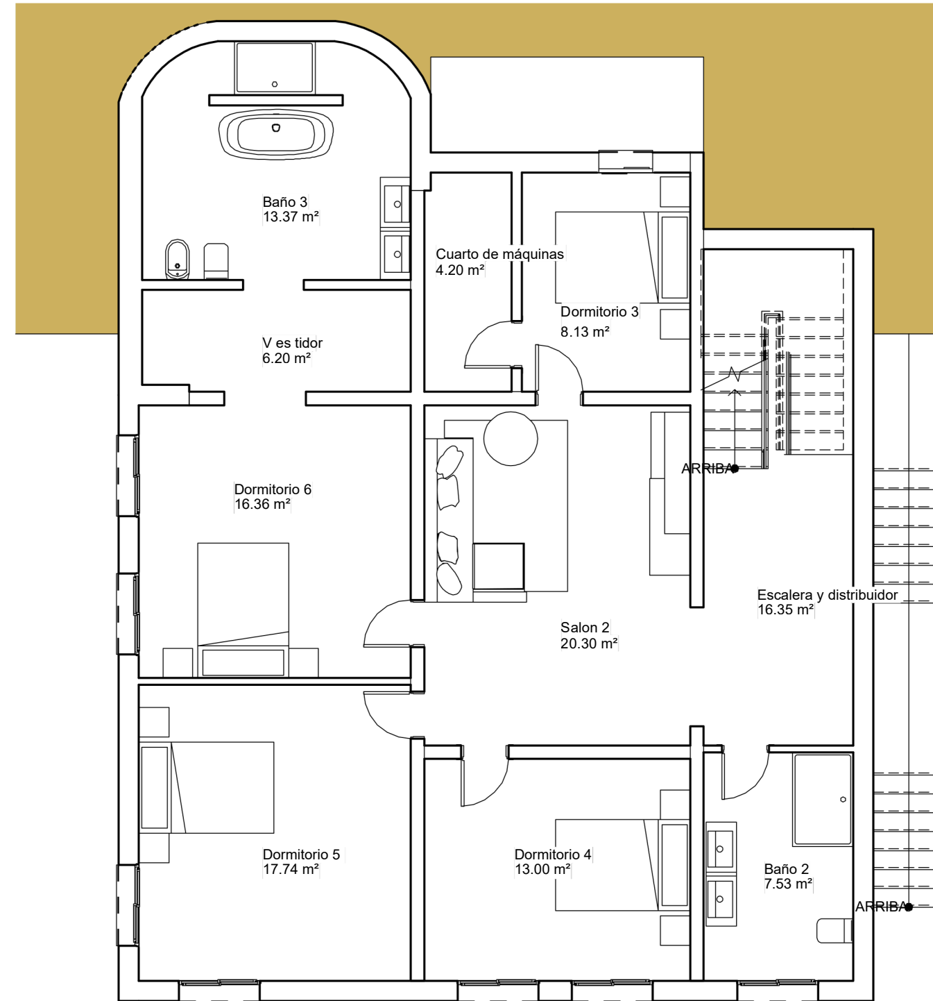
Mid Floor
