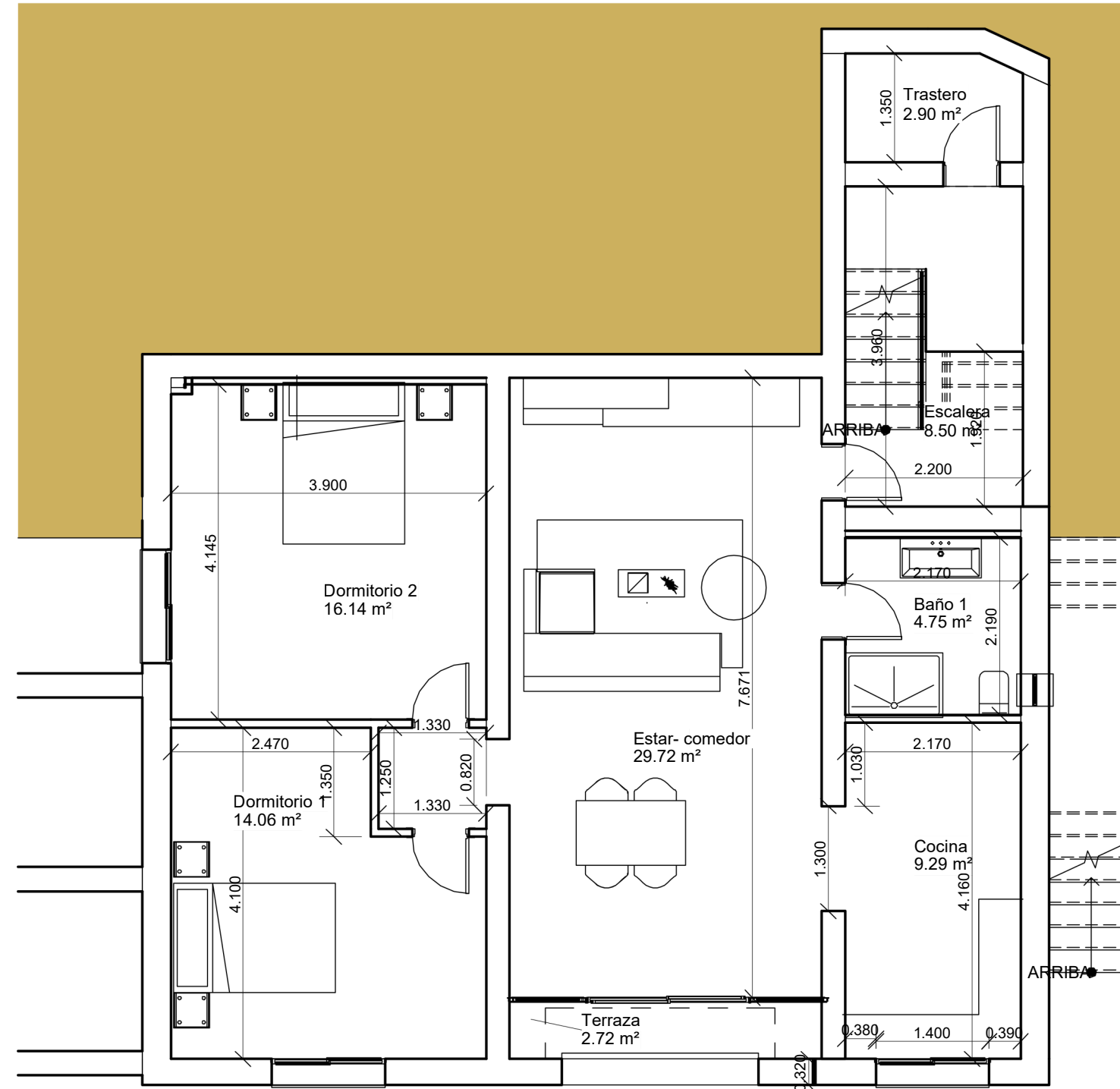
Lower Floor
