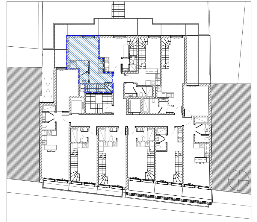
Floor plan 3
