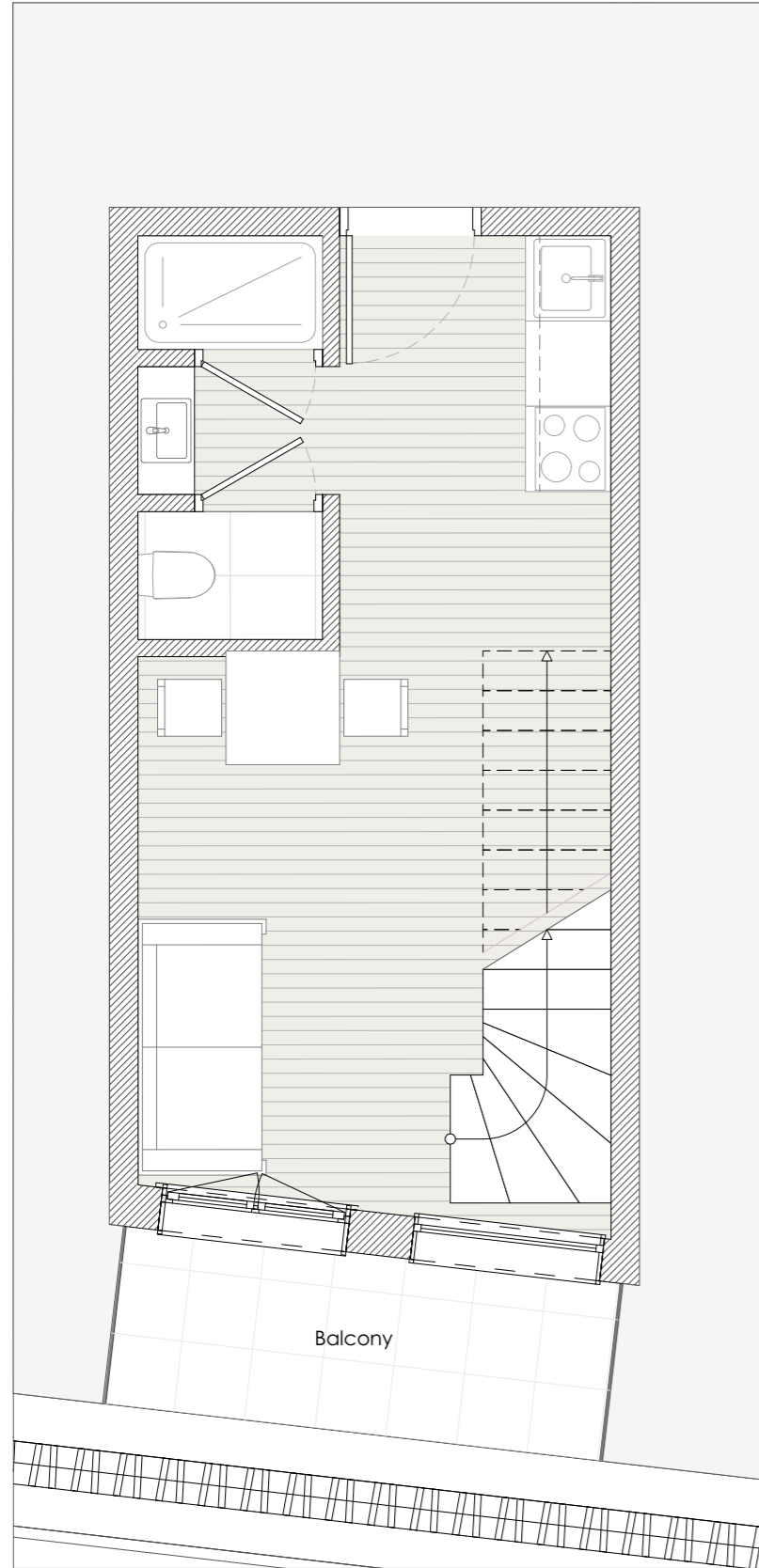
Floor plan - AP21 3th Floor
