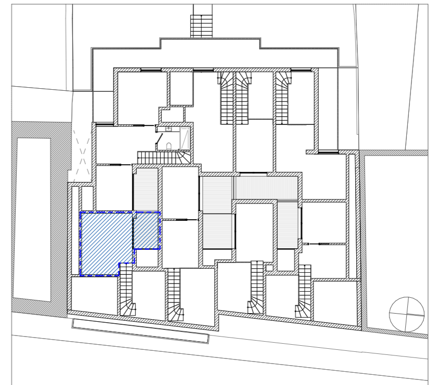
Floor plan 4
