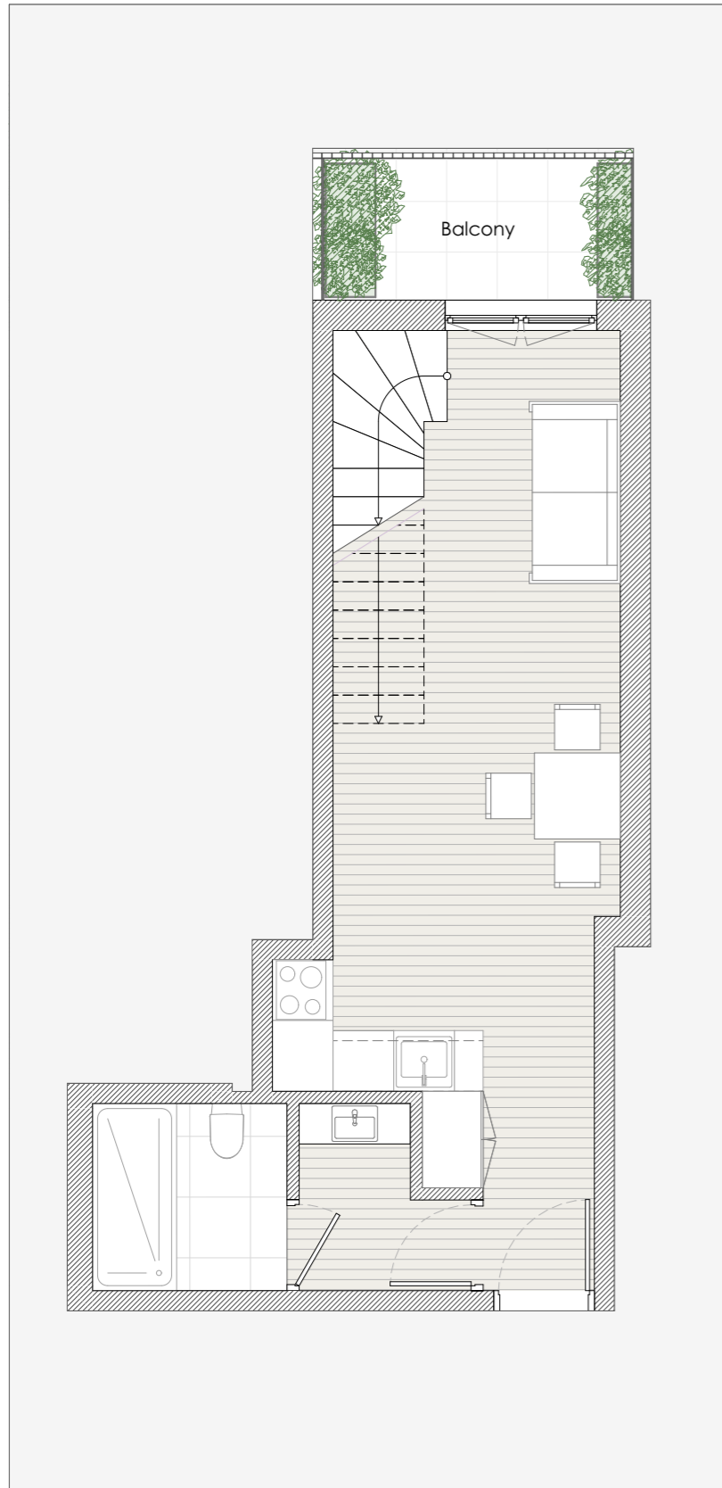
Floor plan - AP23 3th Floor
