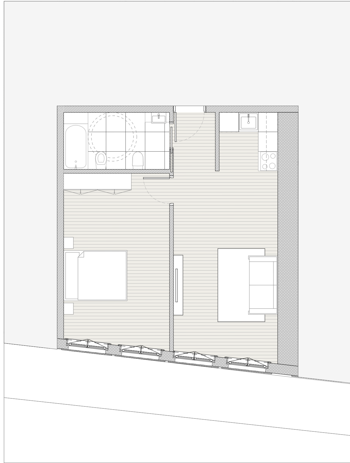
Floor plan - AP12 2nd Floor
