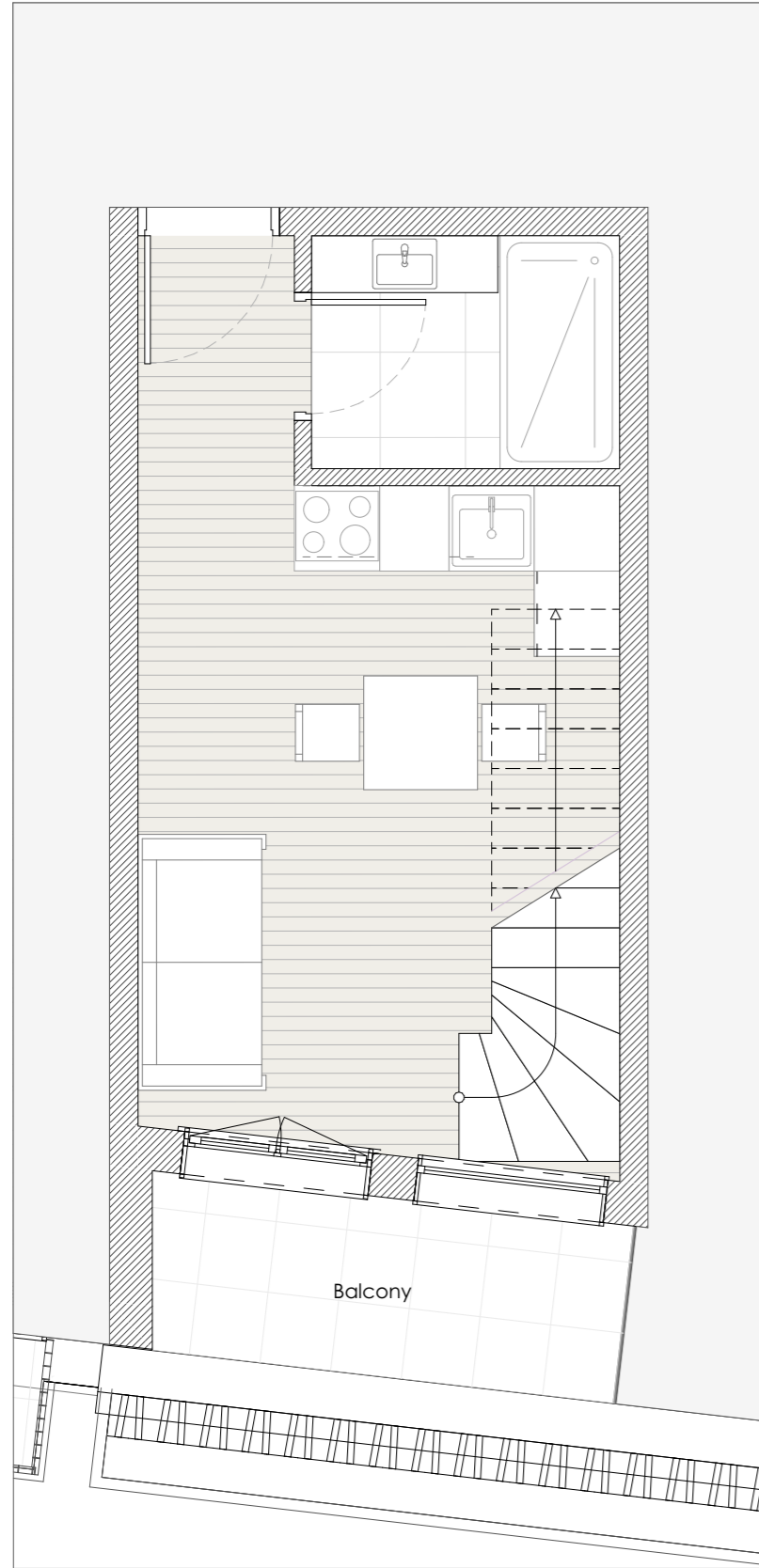
Floor plan - AP20 3th Floor
