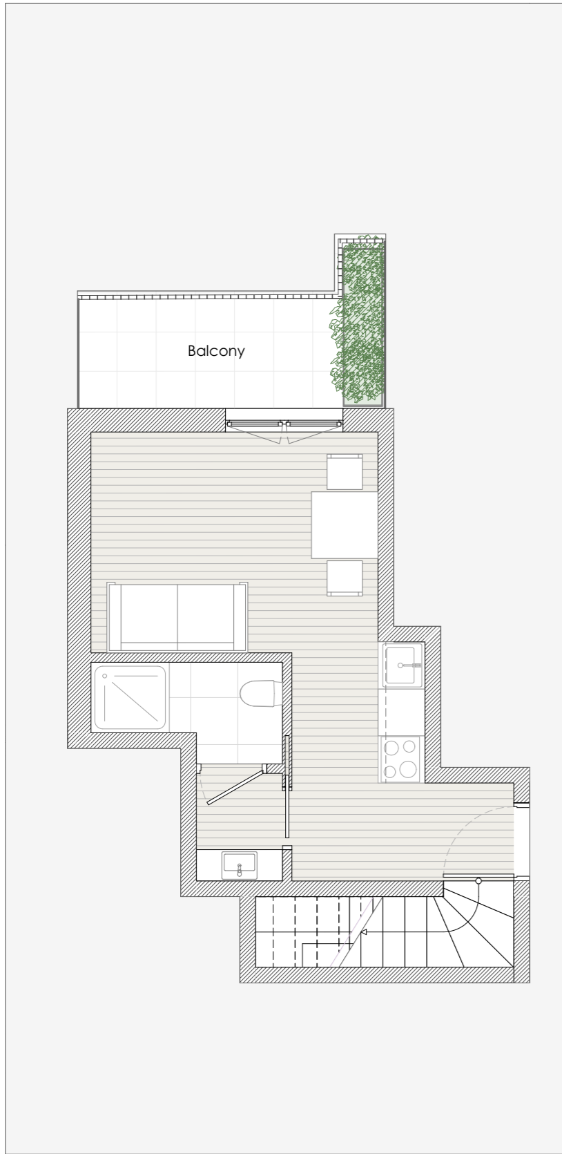
Floor plan - AP26 3th Floor
