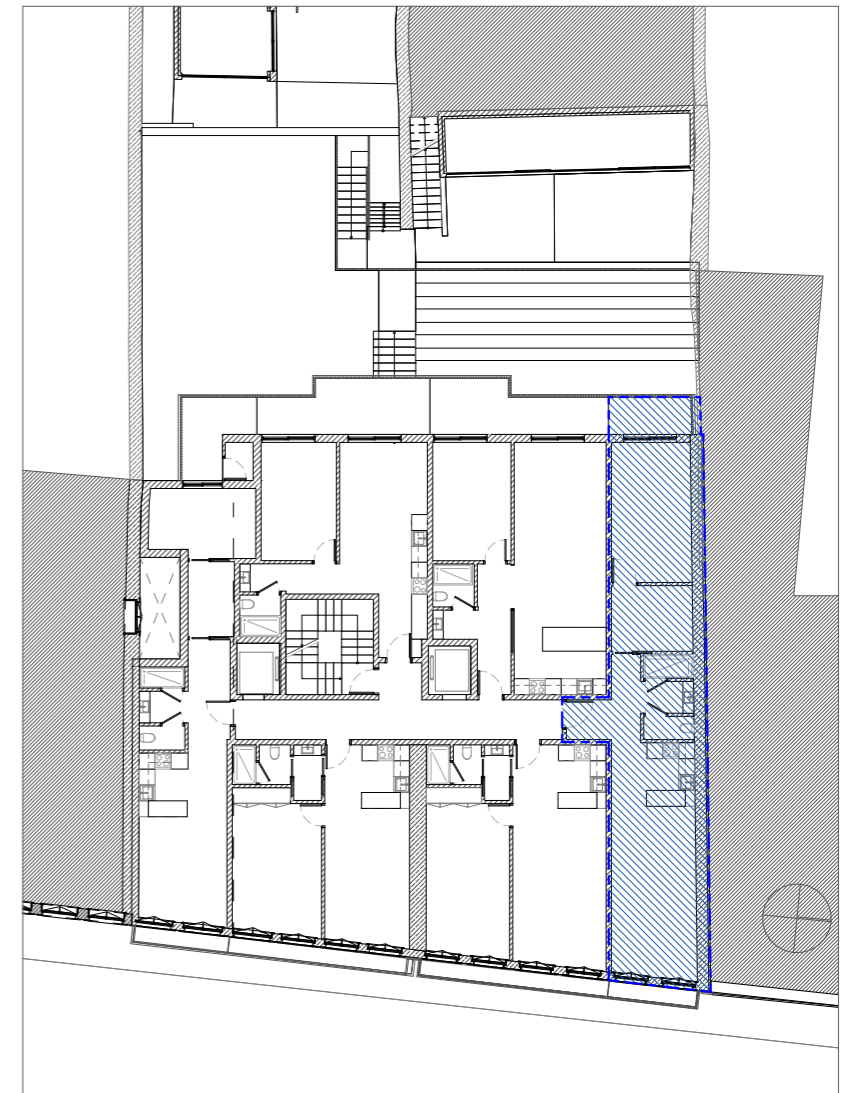
Floor plan 2
