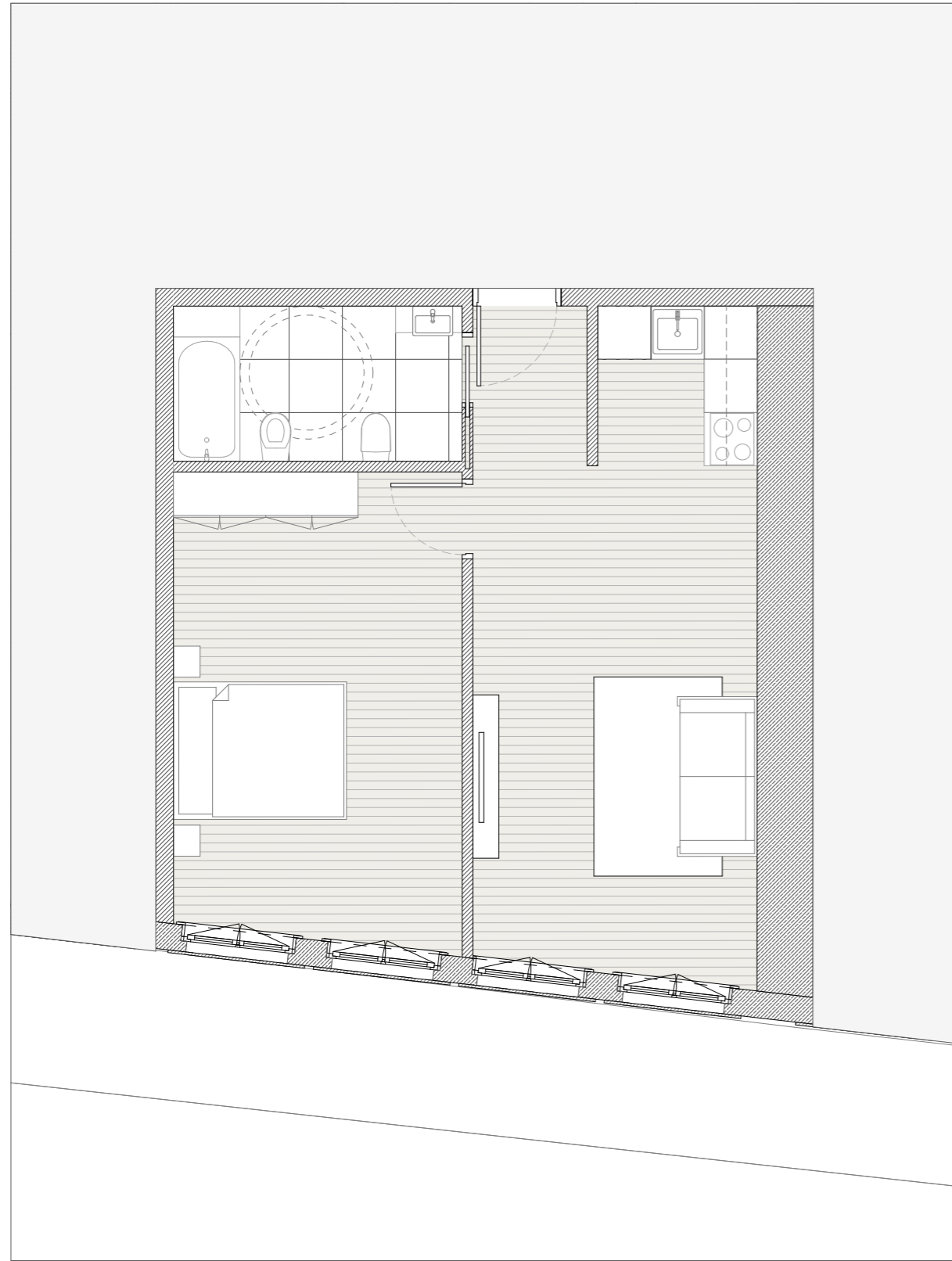
Floor plan - AP06 1st Floor
