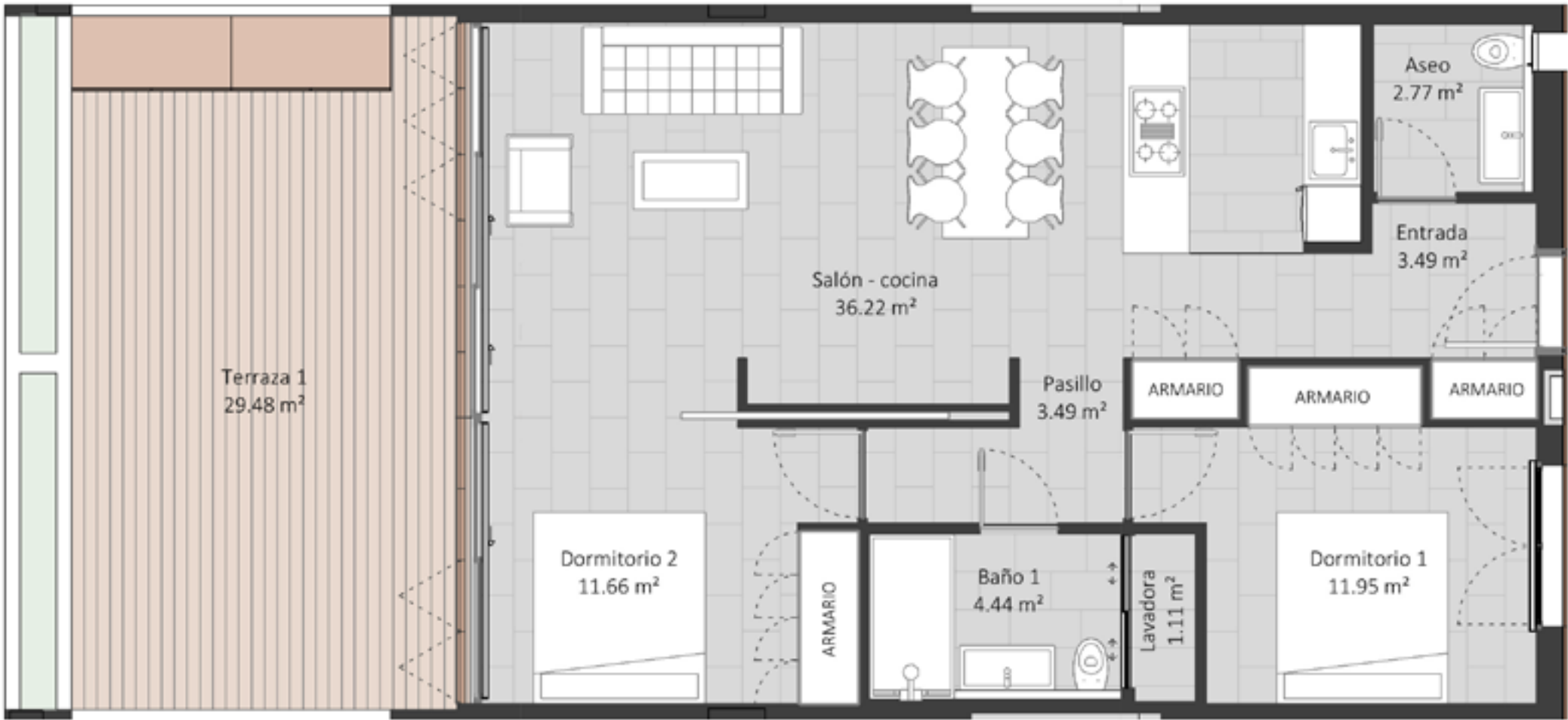
Planta Baja / GROUND FLOOR
