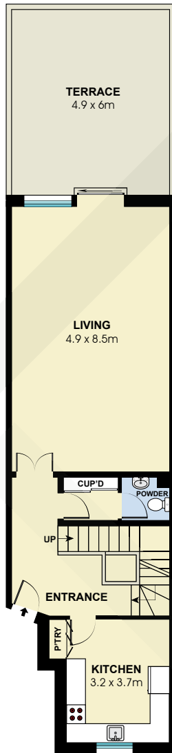
Ground Floor
